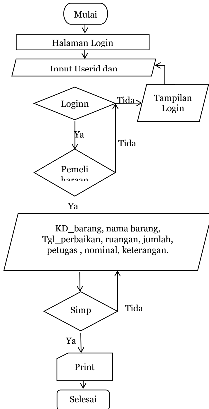
Gambar 5. 3 Diagram Flowchart
